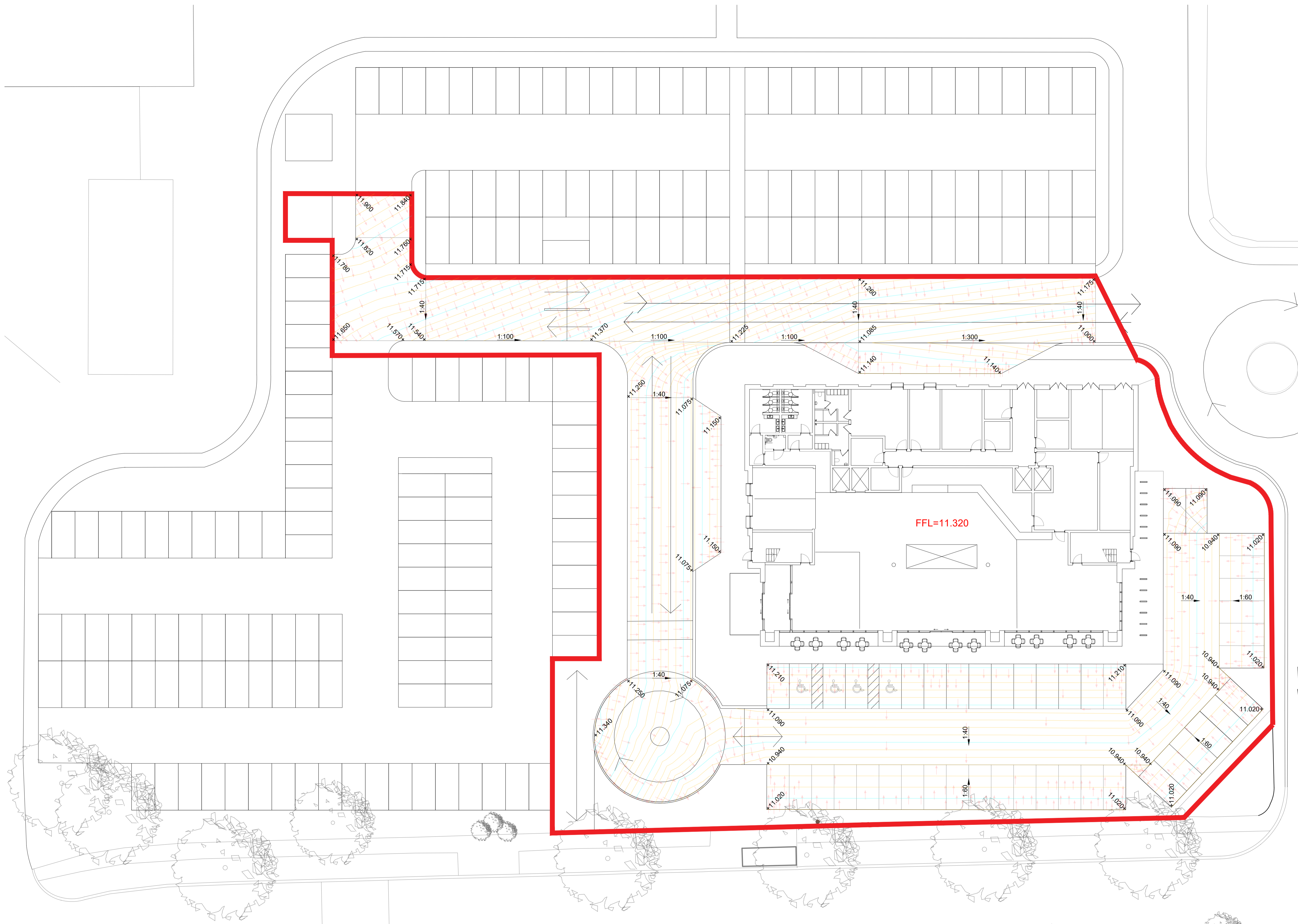
Finished Levels Scale 1:200
